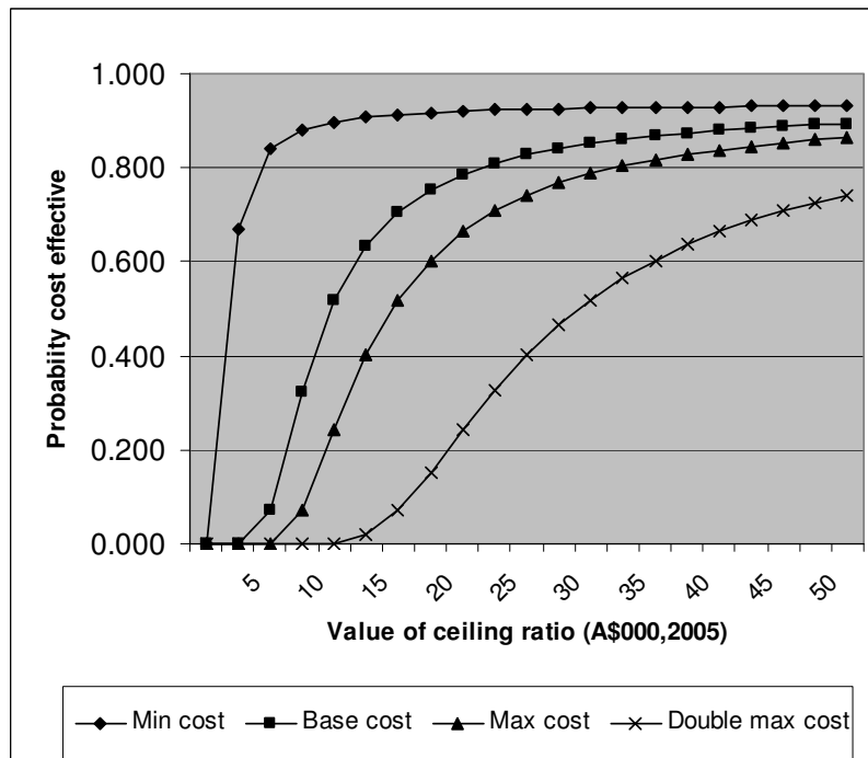
Figure 1 Cost effectiveness acceptability curves
